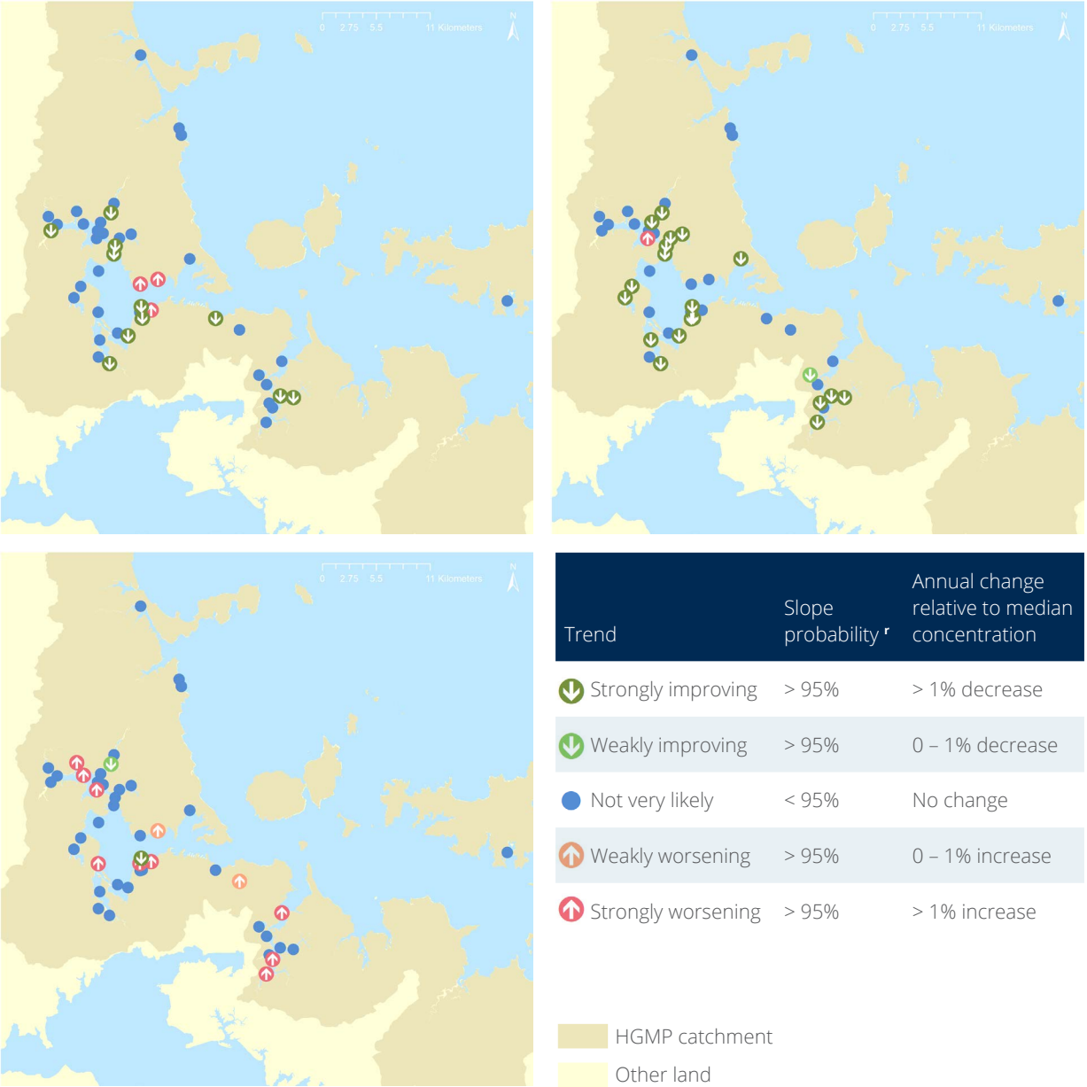
Figure 32: Trends in copper, lead and zinc for sites with sufficient long-term data.
