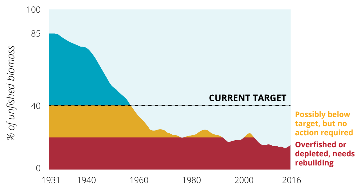
Figure 12: Modelled tarakihi biomass for the entire east coast of Aotearoa. Note that a (relative) biomass target was not defined until 2017, when the first fully quantitative stock assessment was carried out for East Coast tarakihi.
