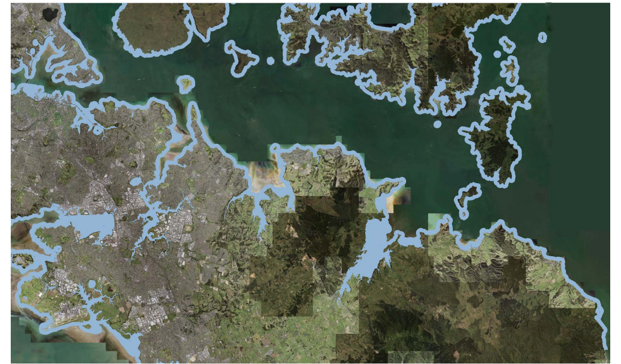
Figure 58: Projected extent of coastal inundation in Auckland with a 1 m sea level rise during a 50-year storm event. Map from https://geomapspublic.aucklandcouncil.govt.nz
