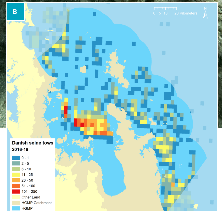
Figure 22: Number of Danish seine sets that occurred between a) 1996-97 to 1998-99, and b) 2016-17 to 2018-19 (data provided by Fisheries NZ).
