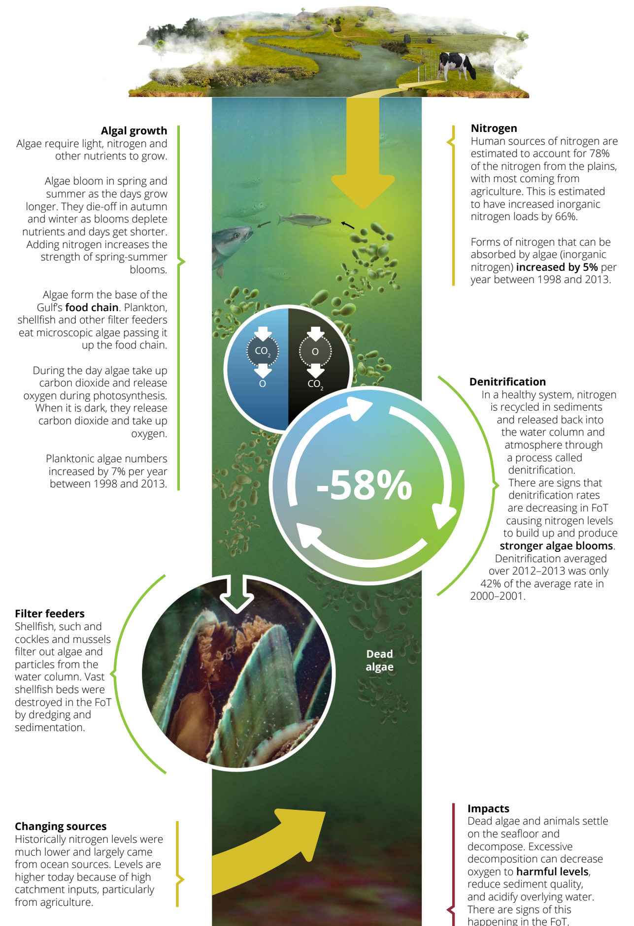
Figure 40. Signs of nitrogen effects in the Firth of Thames (FoT)
