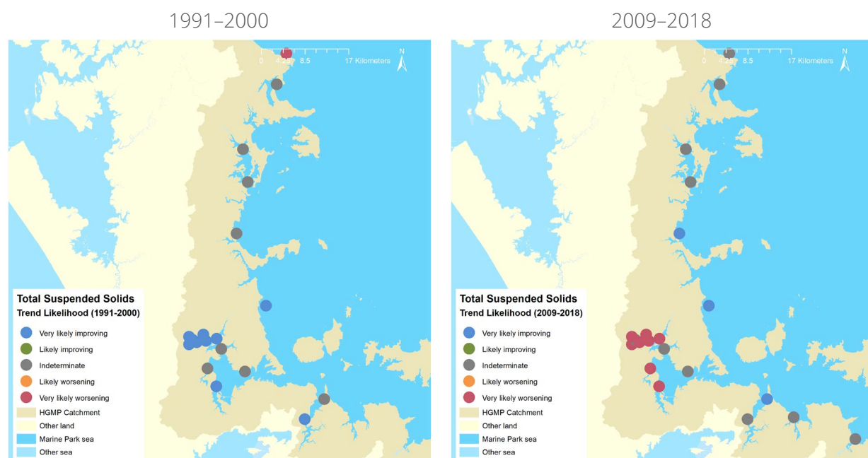
Figure 52: Trends in total suspended solid concentrations between 1991–00 and 2009–2018.
