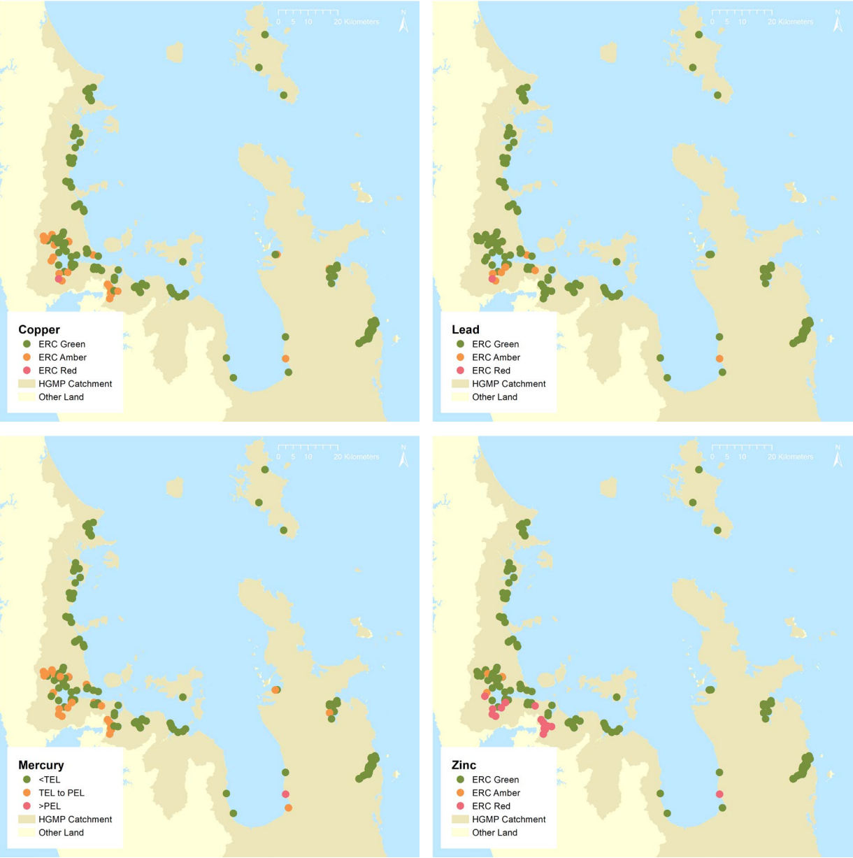
Figure 31: Most recent monitoring results available for each site in the Marine Park showing the ERC status of sites for copper, lead and zinc; and Effects Level status for mercury (unlikely (green), threshold effects level (amber, TEL=0.13 mg/kg) and probable effects level (red, PEL=0.71 mg/kg)). For four sites the most recent data was obtained between 2007 and 2009. For the other 156 sites, the most recent data was obtained since 2010.
