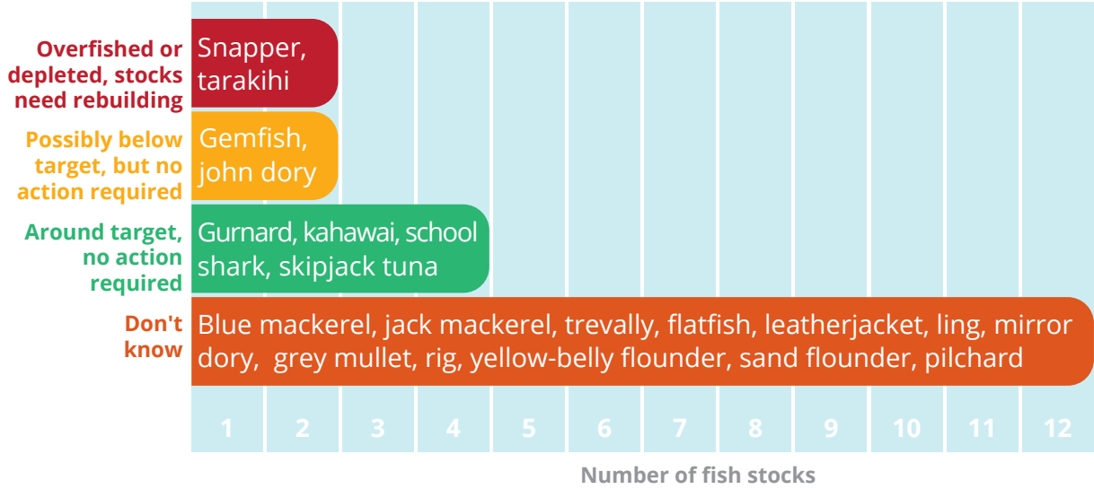
Figure 10: Status of the top 20 fish stocks caught commercially in the Marine Park in relation to the targets set by the Minister of Fisheries.
