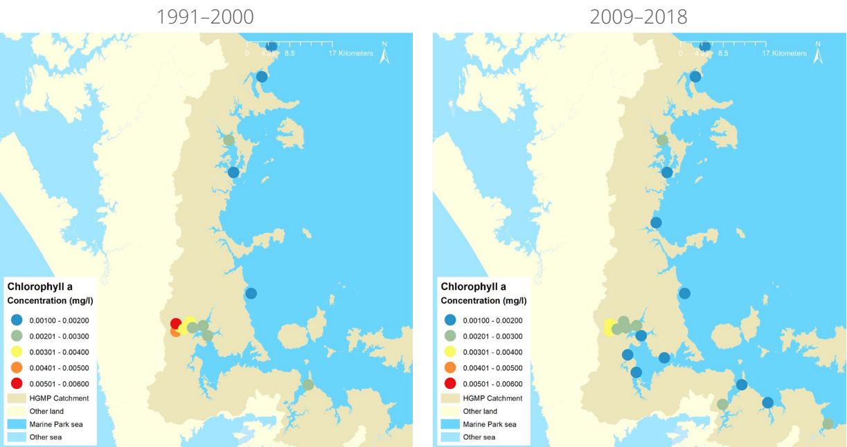
Figure 36: Median total chlorophyll a concentrations at monitored coastal sites between 1991–00 and 2009–18.
