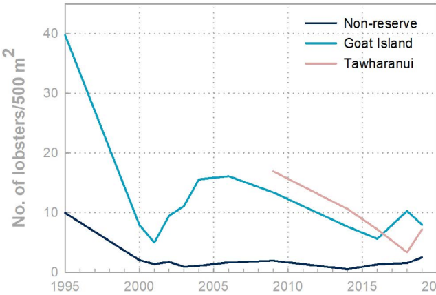
Figure 15: Counts of kōura in Leigh and Tāwharanui marine reserves and nearby non-reserve areas.
