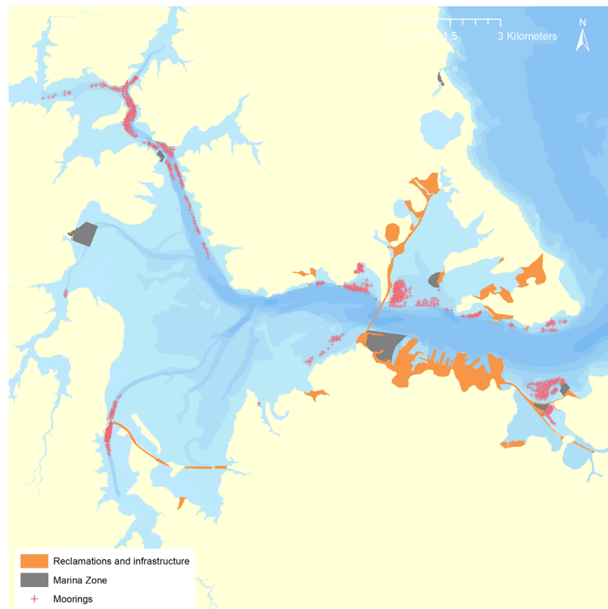
Figure 27: Key coastal sprawl features in the Waitematā Harbour. Data provided by Auckland Council, Auckland Transport and adapted from “Entrances to Auckland harbour” Hydrographic Office of the Admiralty 1857.
