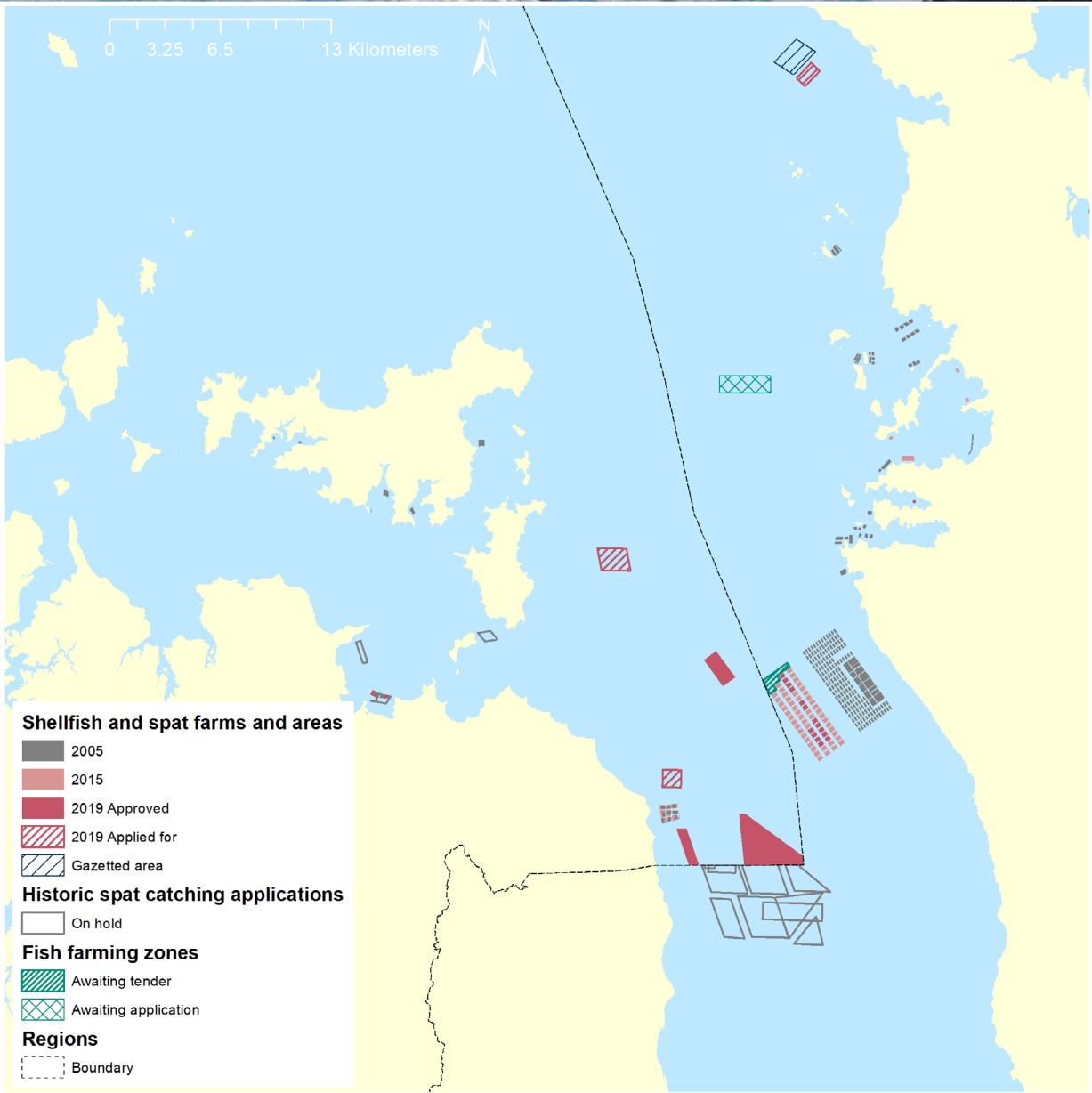
Figure 26: Current and potential aquaculture areas in the Firth of Thames and inner Marine Park.
